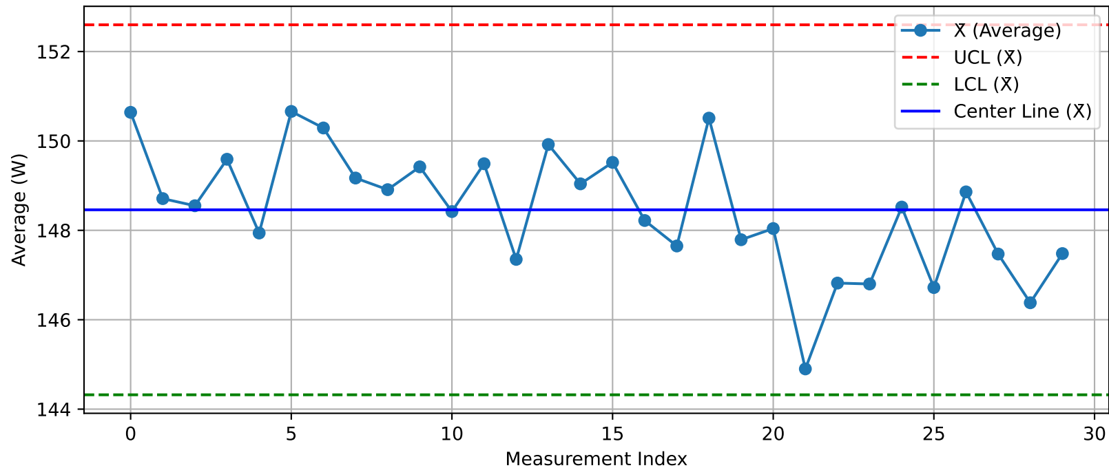
DUT - \bar{X} Chart (T9@Test2.xlsx)
