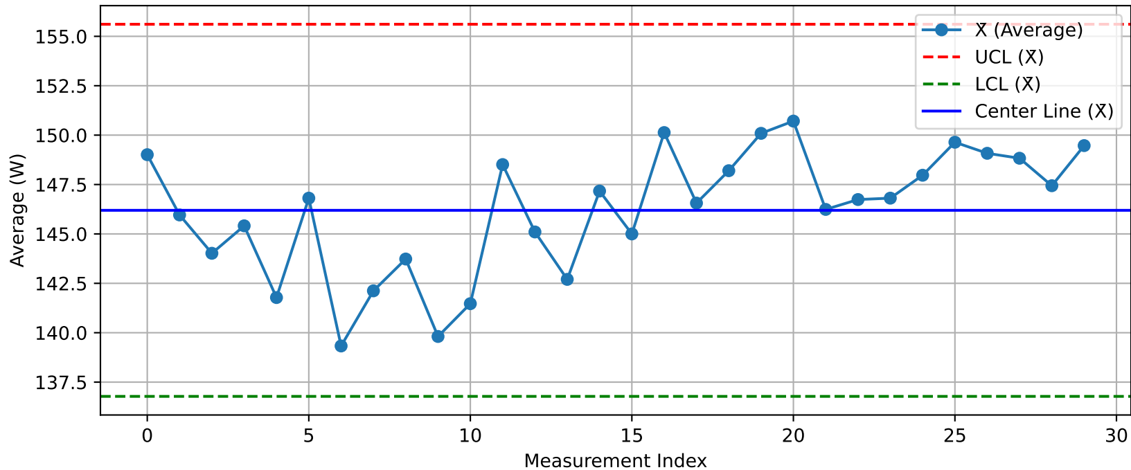
DUT - \bar{X} Chart (T9@Test2_Nuitka.xlsx)
