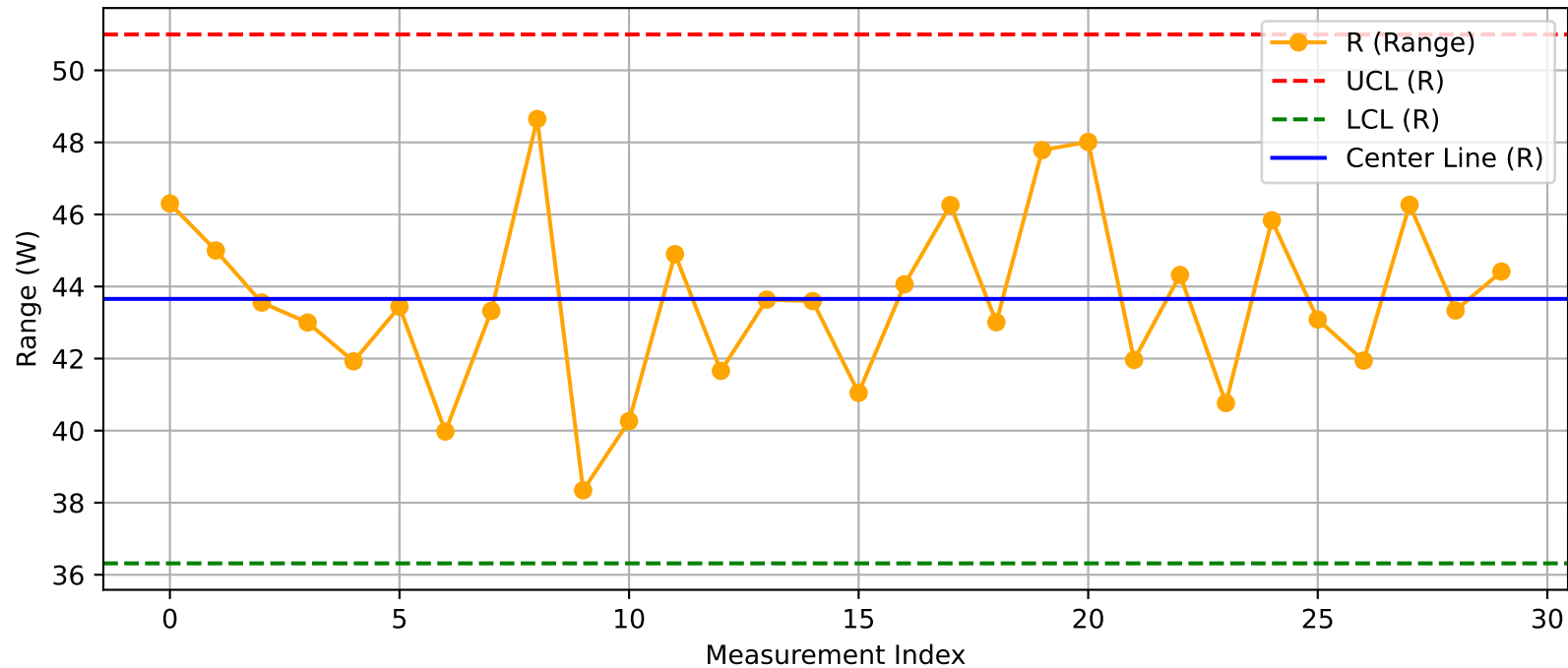
DUT - R Chart (T05_Test103@Test.xlsx)
