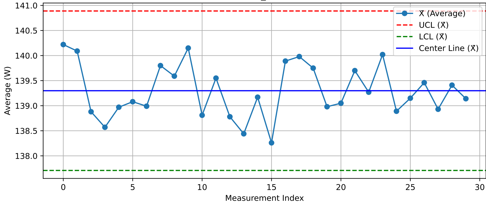
DUT - \bar{X} Chart (T05_Test103@Test.xlsx)
