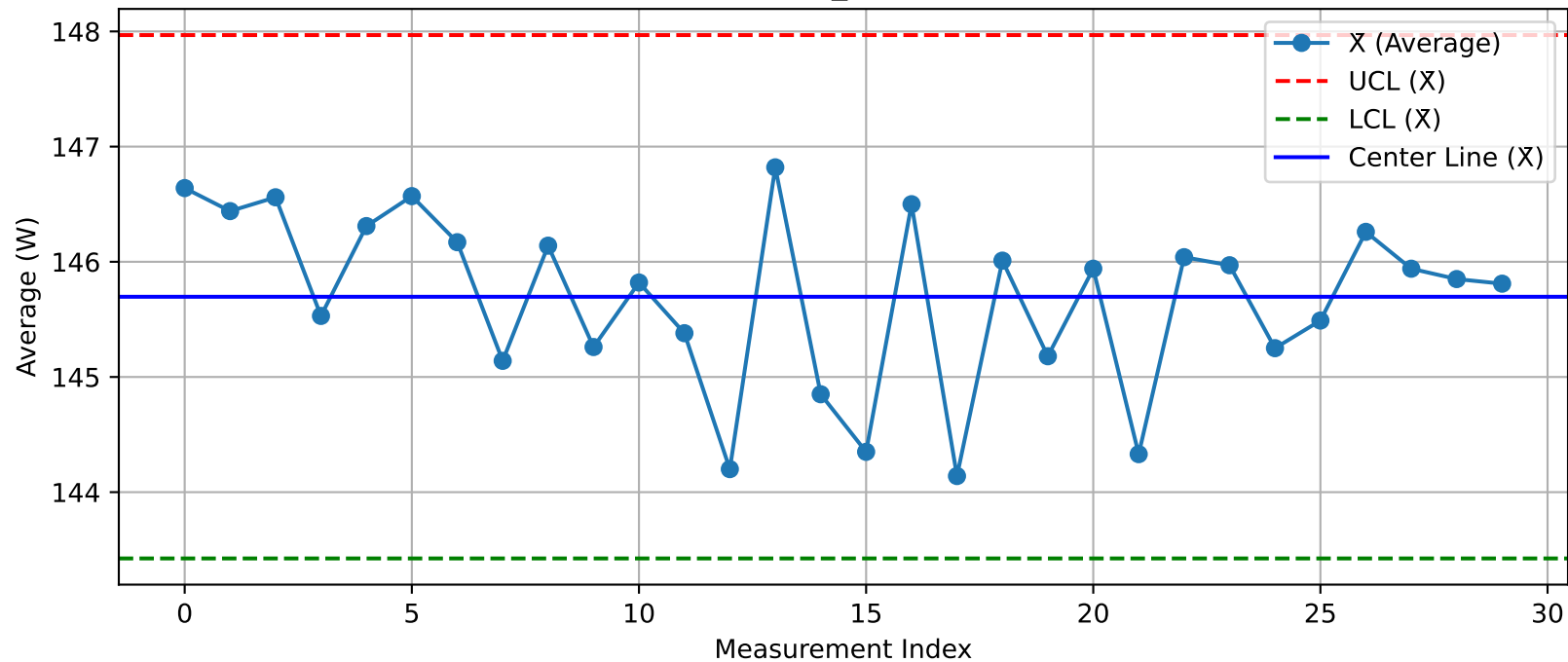
DUT - \bar{X} Chart (T05_Test2O3@Test.xlsx)
