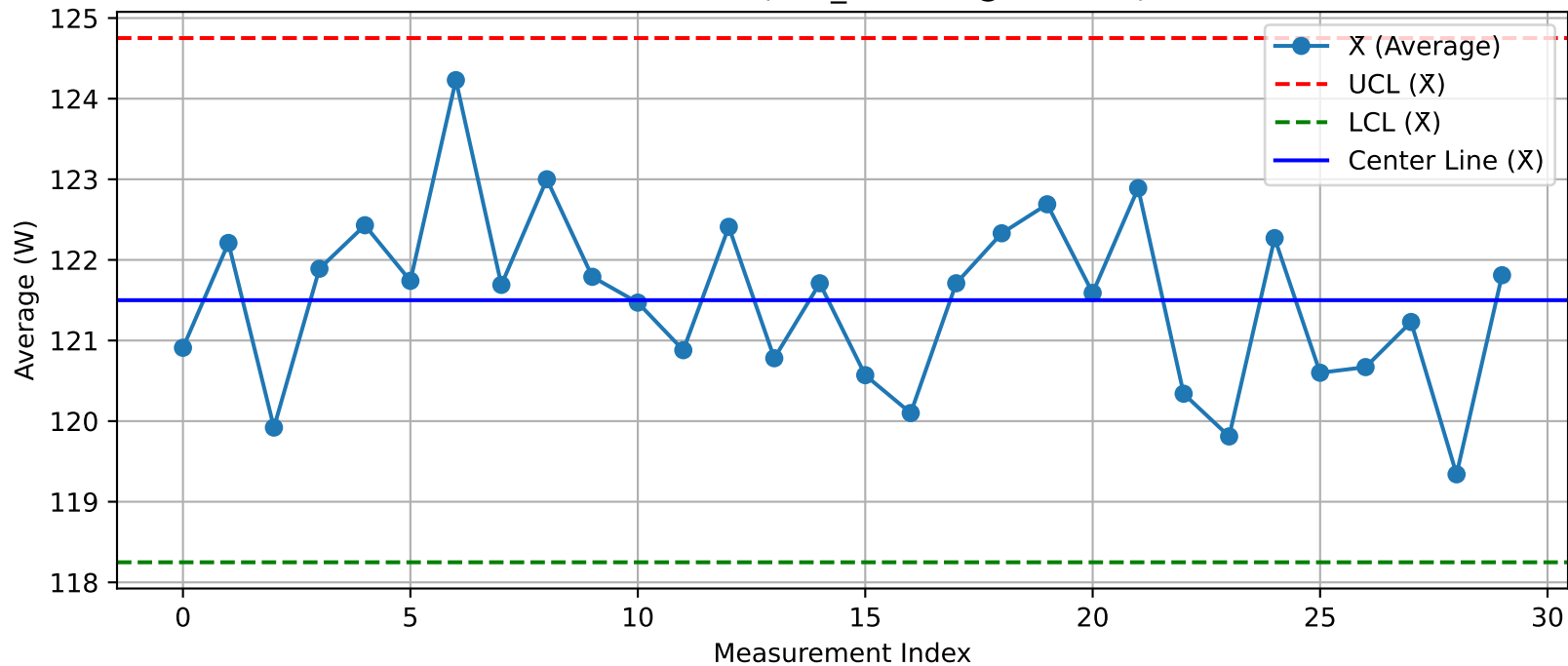
DUT - \bar{X} Chart (T07_Test100@Test.xlsx)
