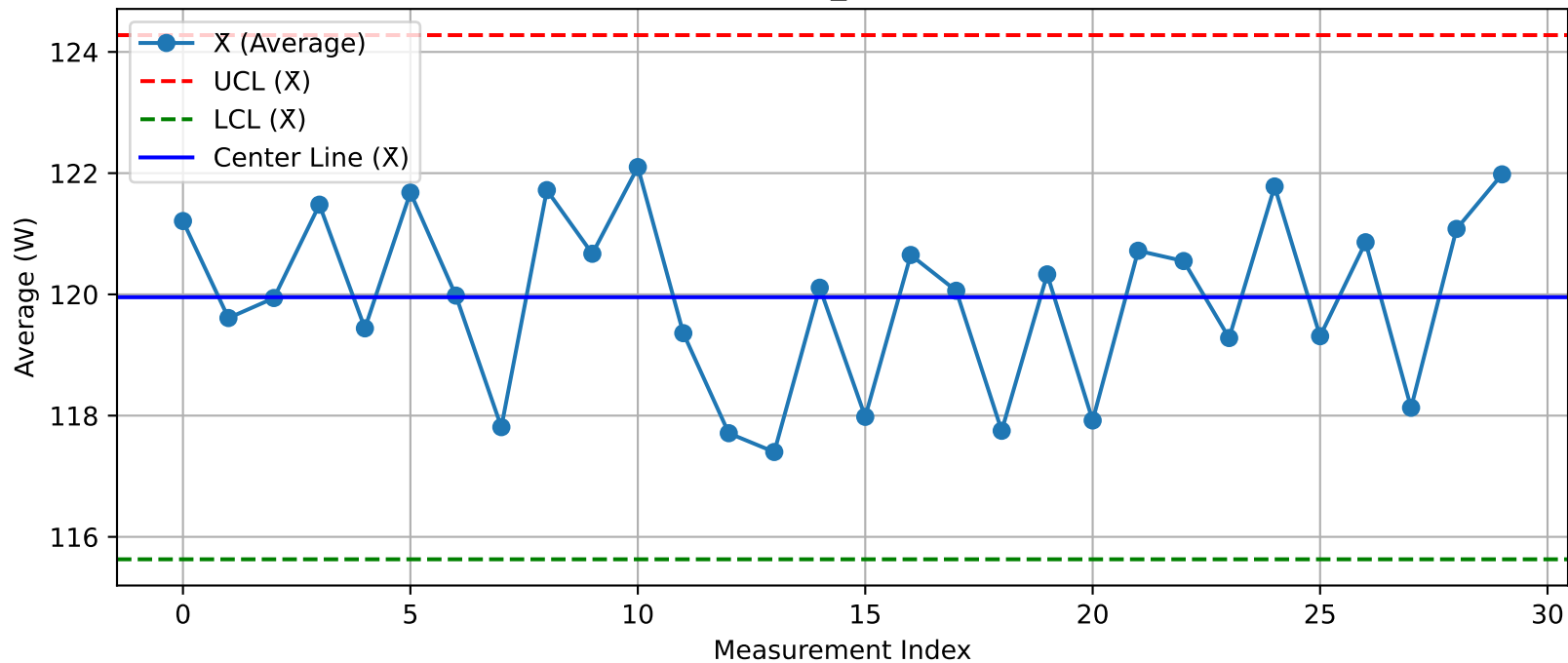
DUT - \bar{X} Chart (T07_Test1O3@Test.xlsx)
