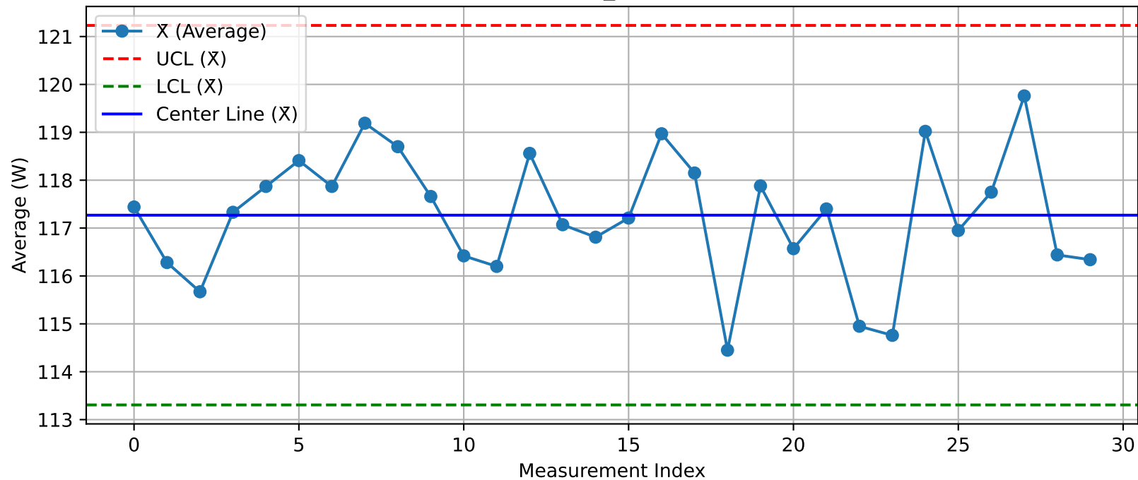
DUT - \bar{X} Chart (T07_Test200@Test.xlsx)
