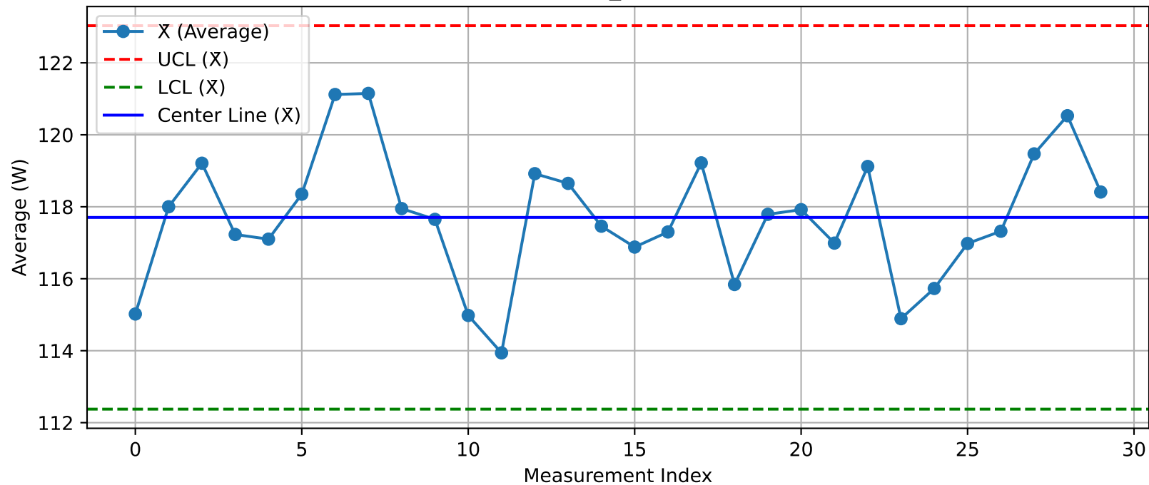
DUT - \bar{X} Chart (T09_Test200@Test.xlsx)
