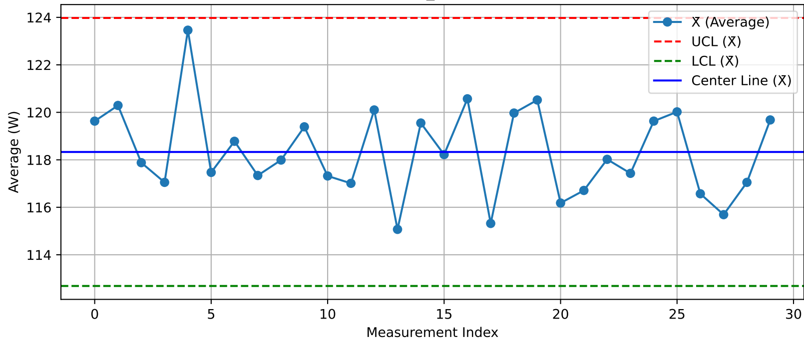
DUT - \bar{X} Chart (T09_Test203@Test.xlsx)
