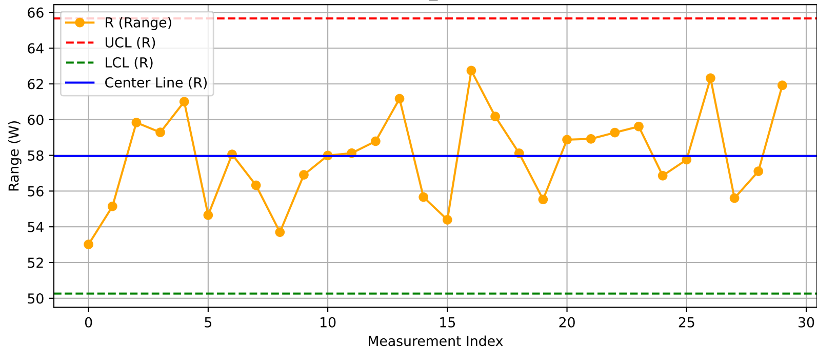
DUT - R Chart (T10_Test100@Test.xlsx)
