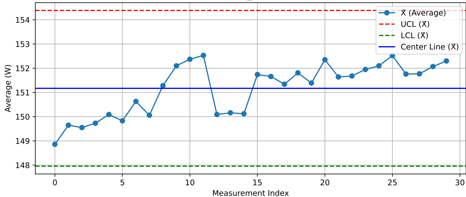
DUT - \bar{X} Chart (T10_Test100@Test.xlsx)
