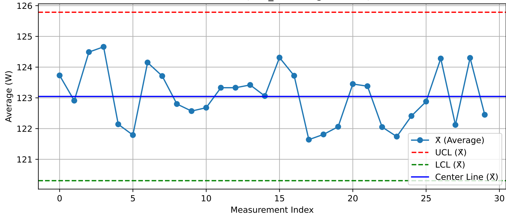
DUT - \bar{X} Chart (T11_Test100@Test.xlsx)
