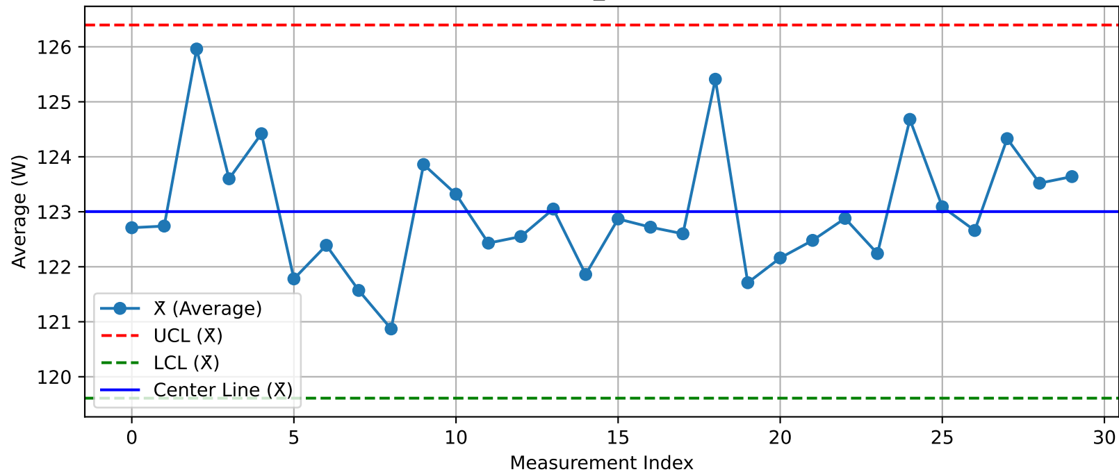
DUT - \bar{X} Chart (T11_Test200@Test.xlsx)
