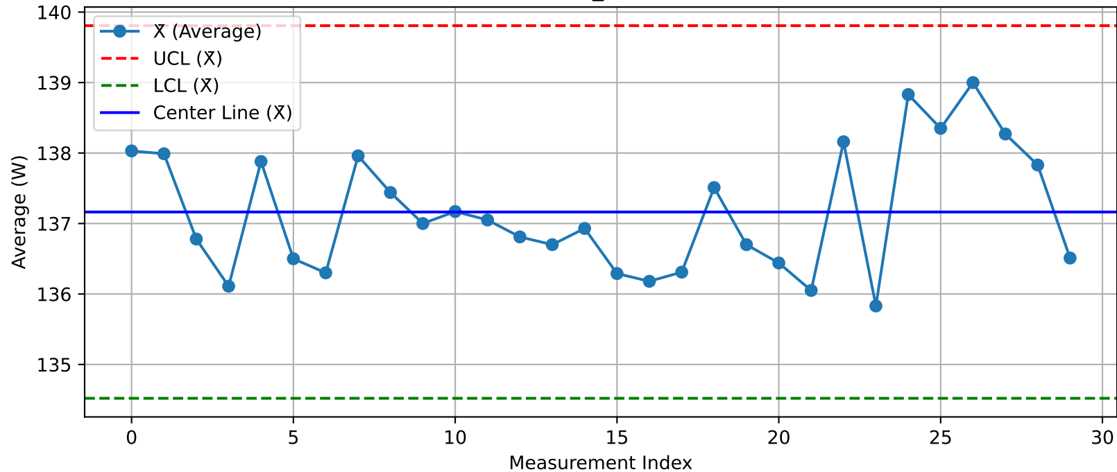
DUT - \bar{X} Chart (T13_Test103@Test.xlsx)
