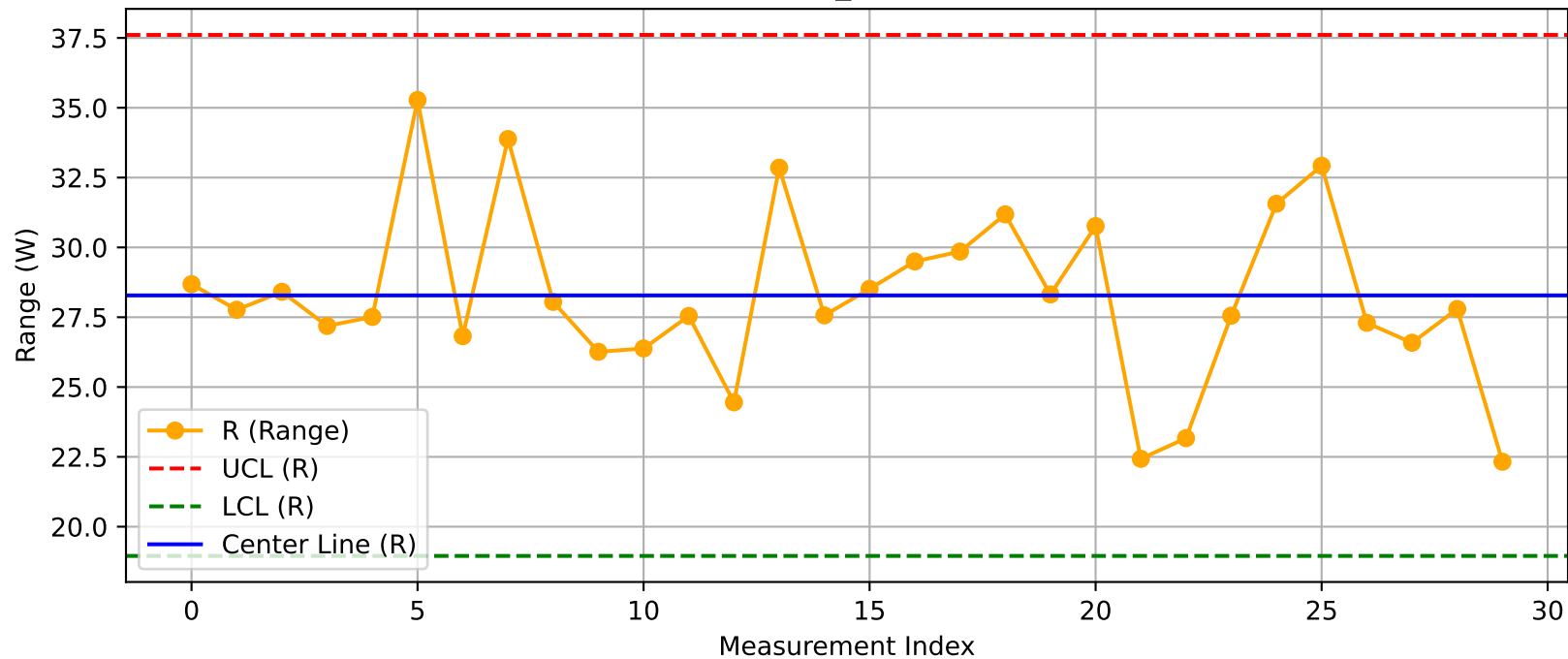
DUT - R Chart (T16_Test103@Test.xlsx)
