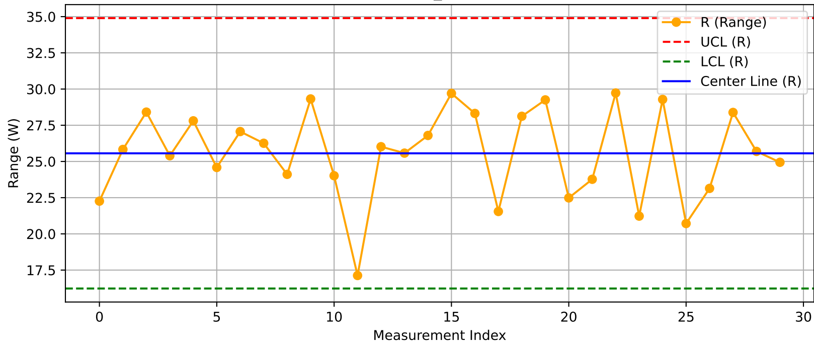
DUT - R Chart (T16_Test200@Test.xlsx)
