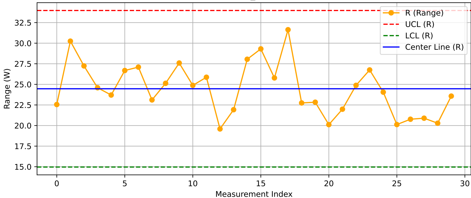
DUT - R Chart (T16_Test203@Test.xlsx)
