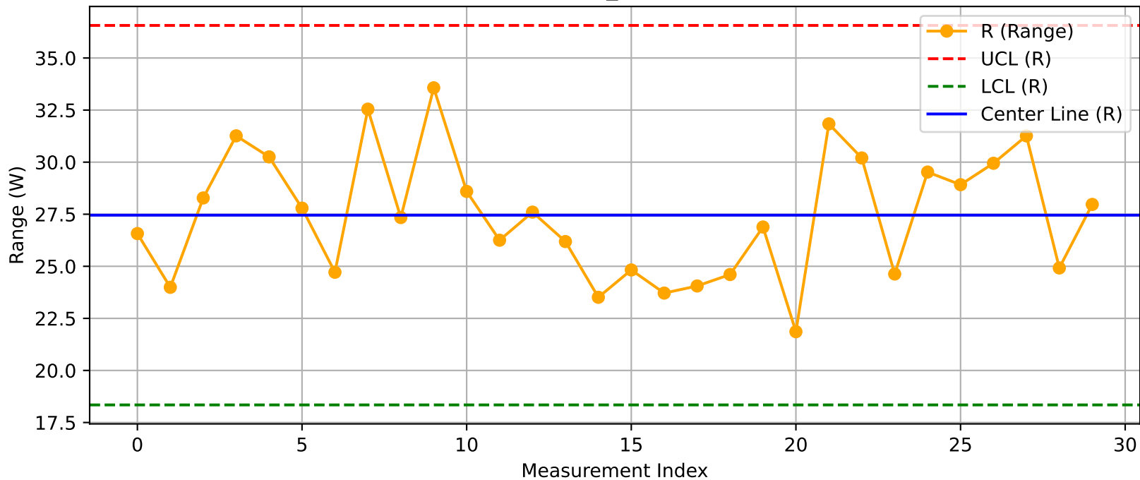
DUT - R Chart (T17_Test1O3@Test.xlsx)
