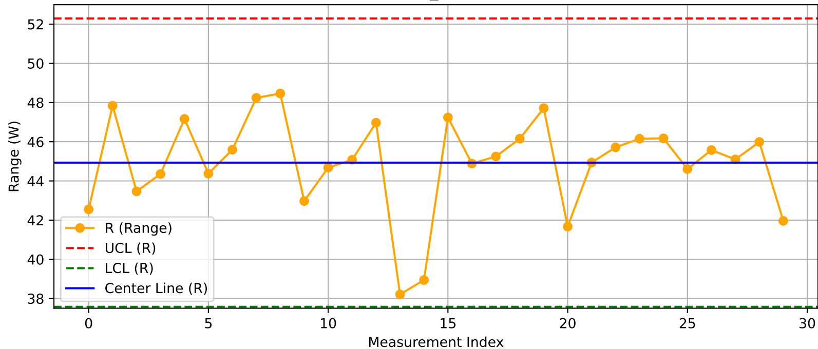
DUT - R Chart (T19_Test200@Test.xlsx)
