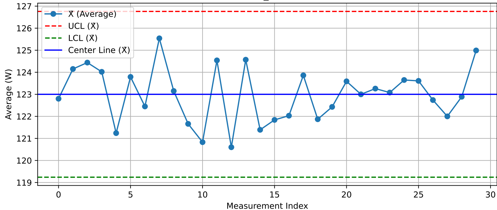
DUT - \bar{X} Chart (T19_Test203@Test.xlsx)
