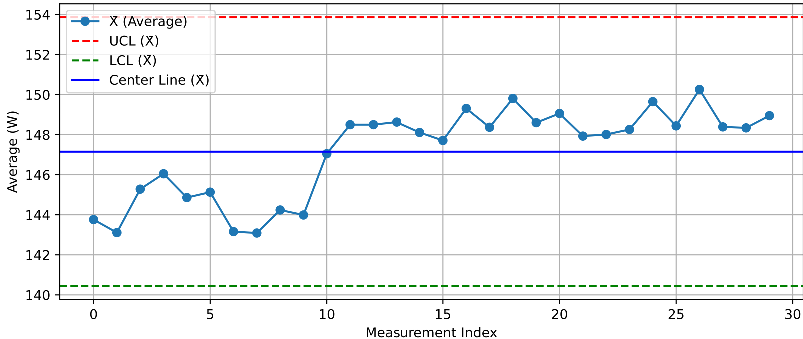
DUT - \bar{X} Chart (T20_Test100@Test.xlsx)
