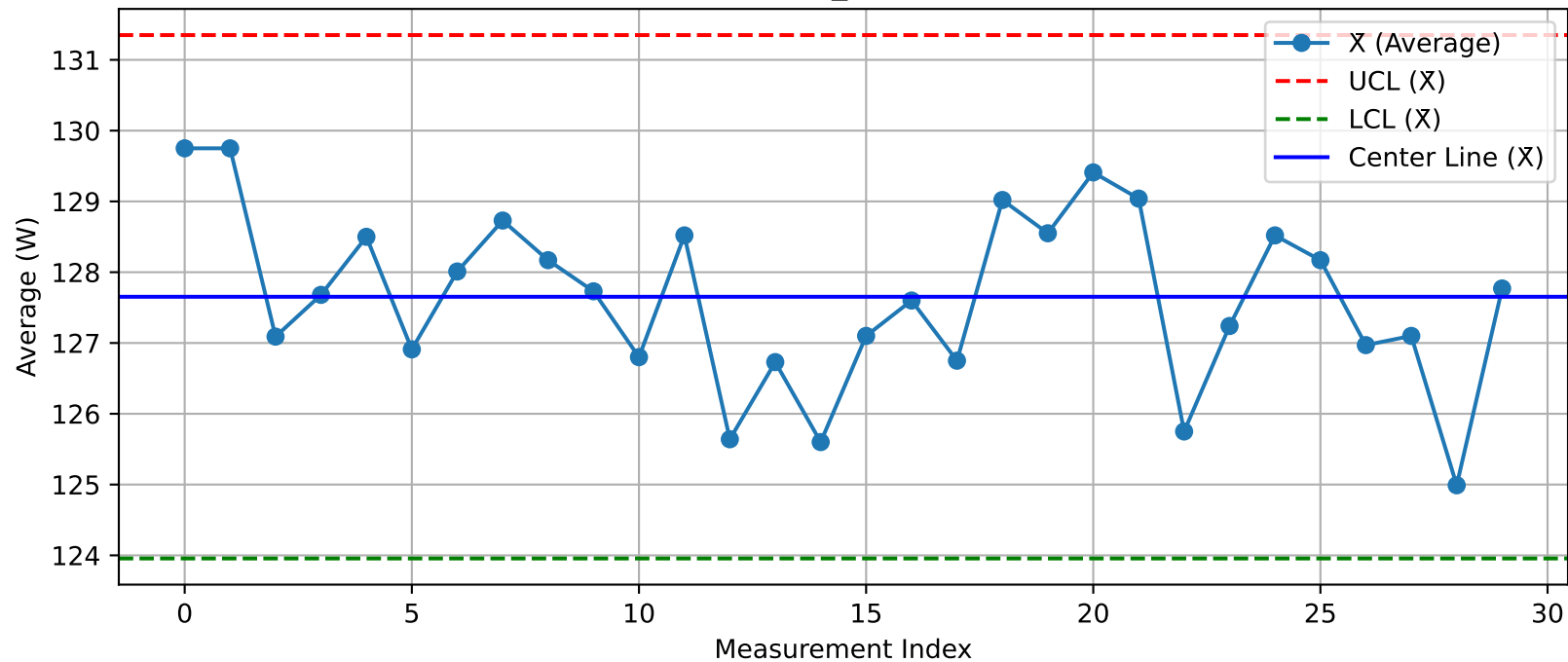
DUT - \bar{X} Chart (T20_Test2O3@Test.xlsx)
