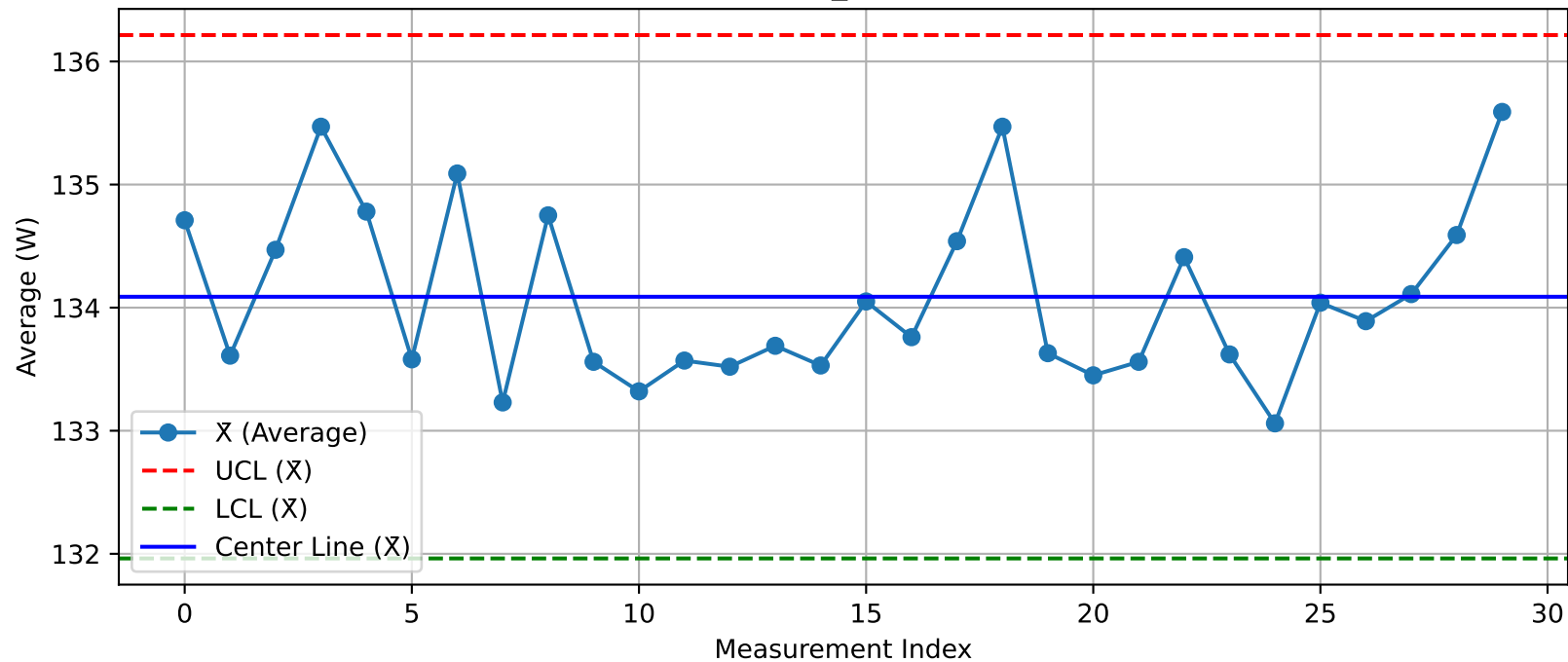
DUT - \bar{X} Chart (T26_Test103@Test.xlsx)
