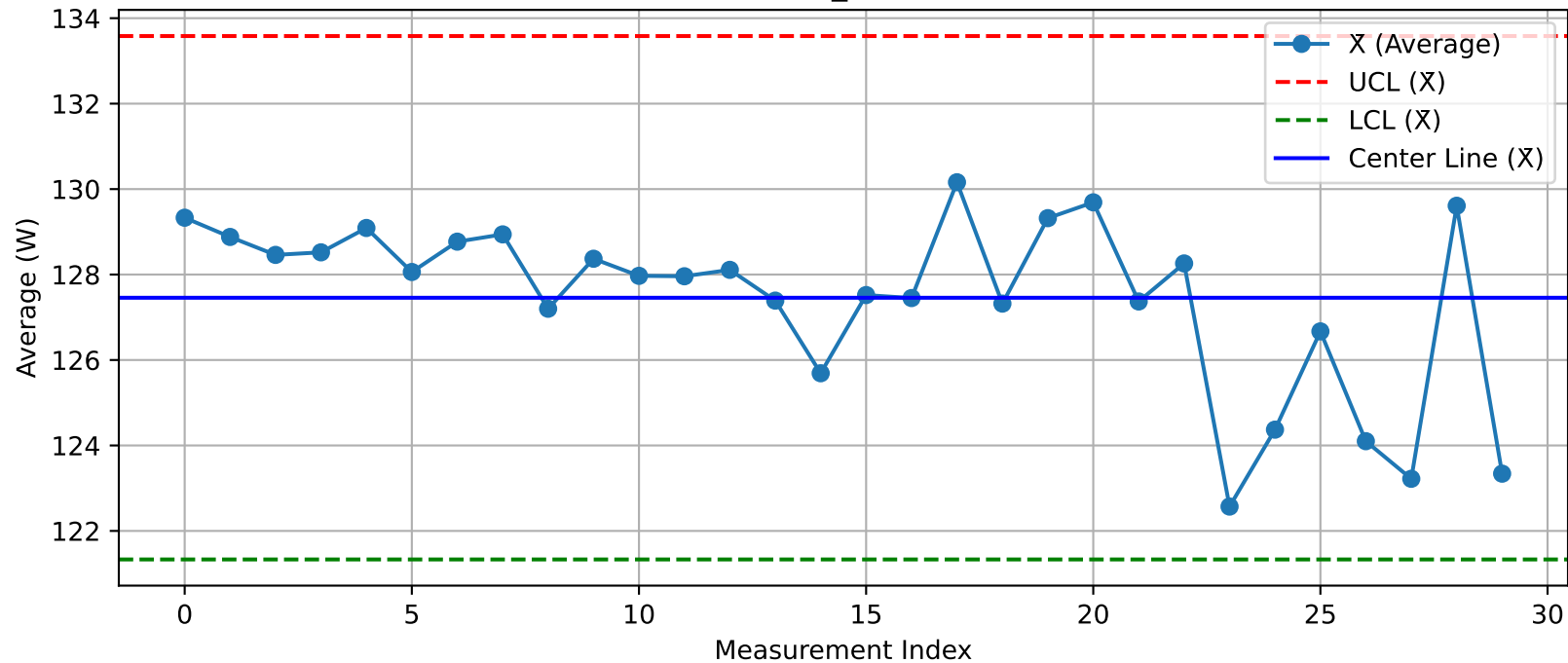
DUT - \bar{X} Chart (T28_Test103@Test.xlsx)
