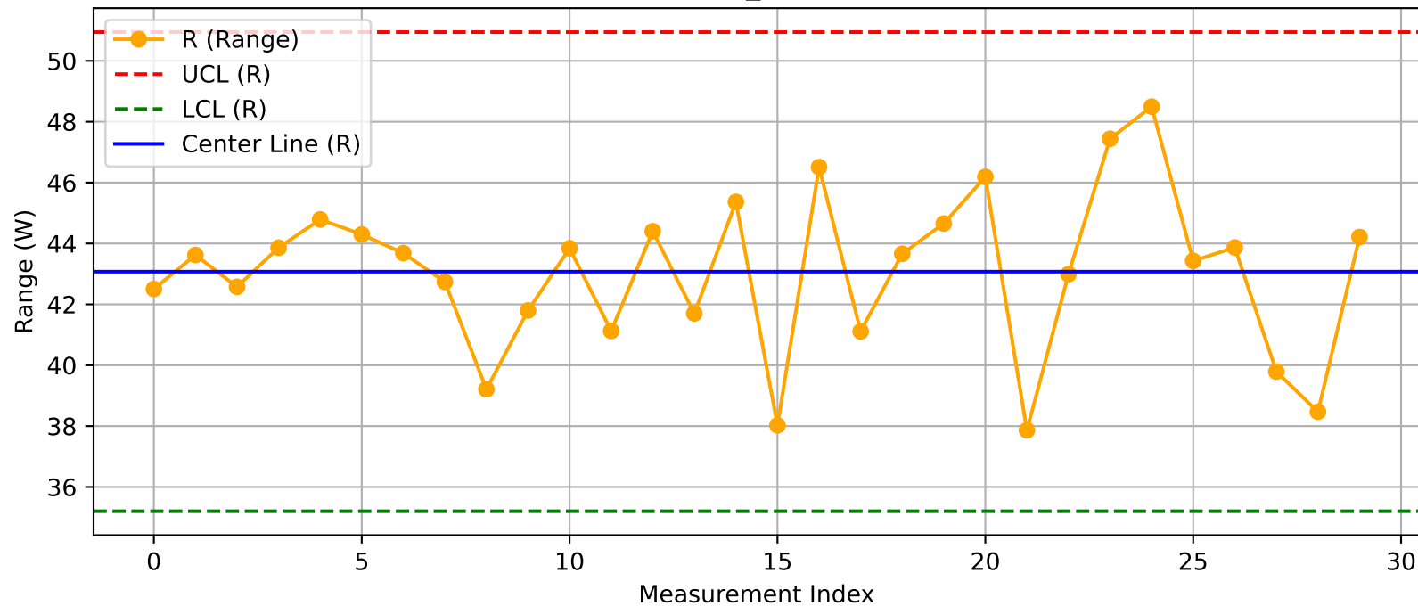
DUT - R Chart (T28_Test203@Test.xlsx)
