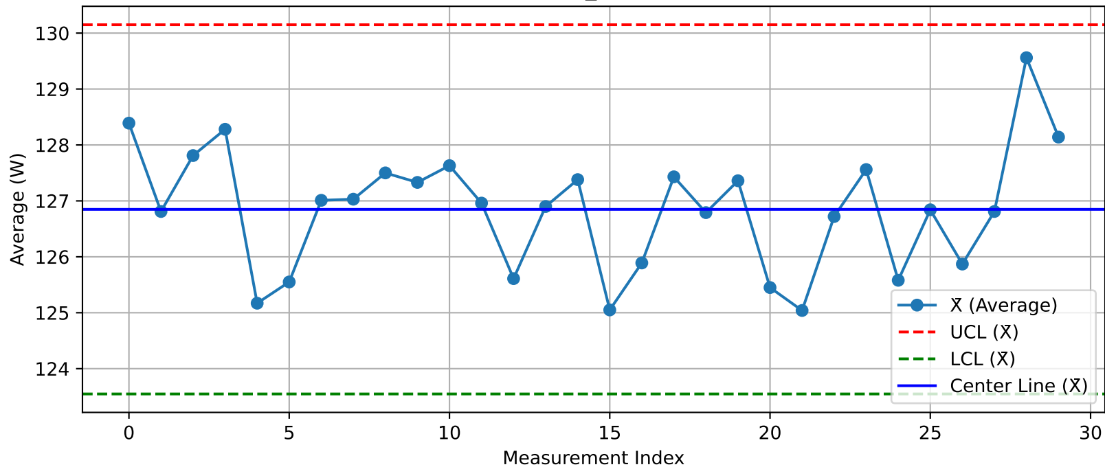
DUT - \bar{X} Chart (T28_Test2O3@Test.xlsx)
