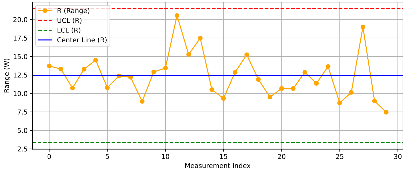
DUT - R Chart (T29_Test200@Test.xlsx)
