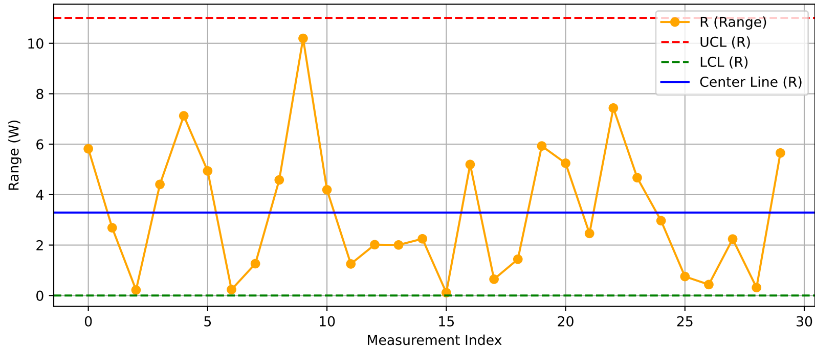
DUT - R Chart (T29_Test203@Test.xlsx)
