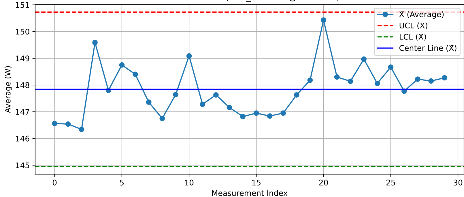
DUT - \bar{X} Chart (T31_Test100@Test.xlsx)
