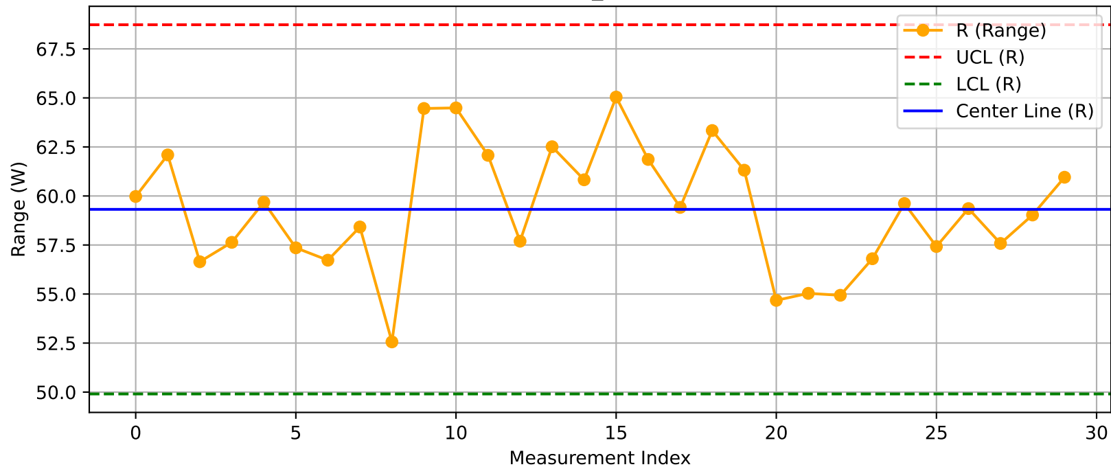
DUT - R Chart (T31_Test103@Test.xlsx)
