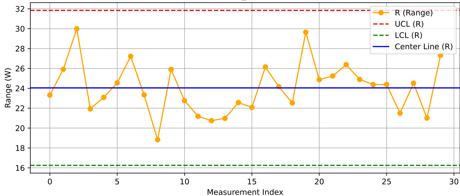
DUT - R Chart (T32_Test100@Test.xlsx)
