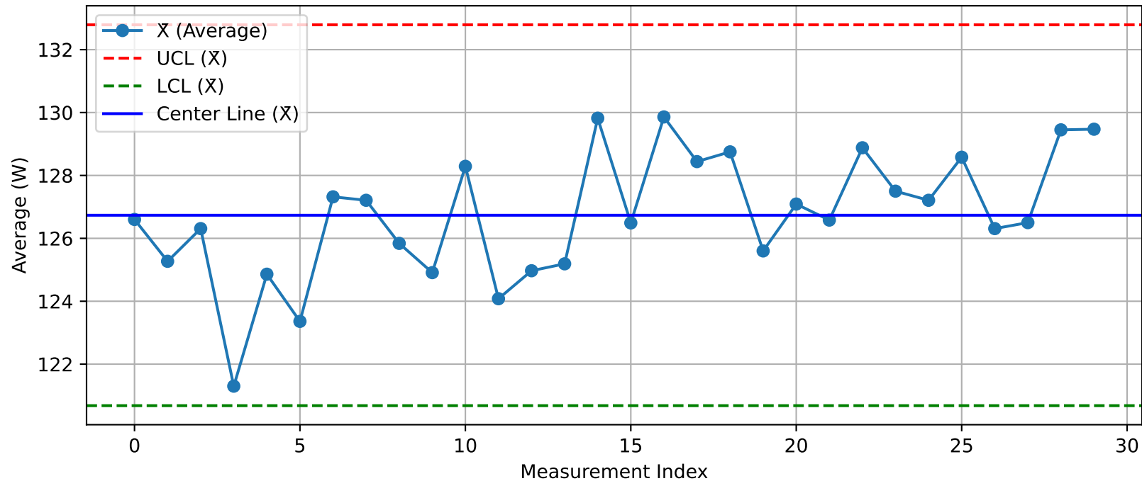
DUT - \bar{X} Chart (T33_Test200@Test.xlsx)
