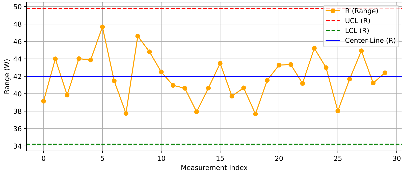
DUT - R Chart (T36_Test200@Test.xlsx)
