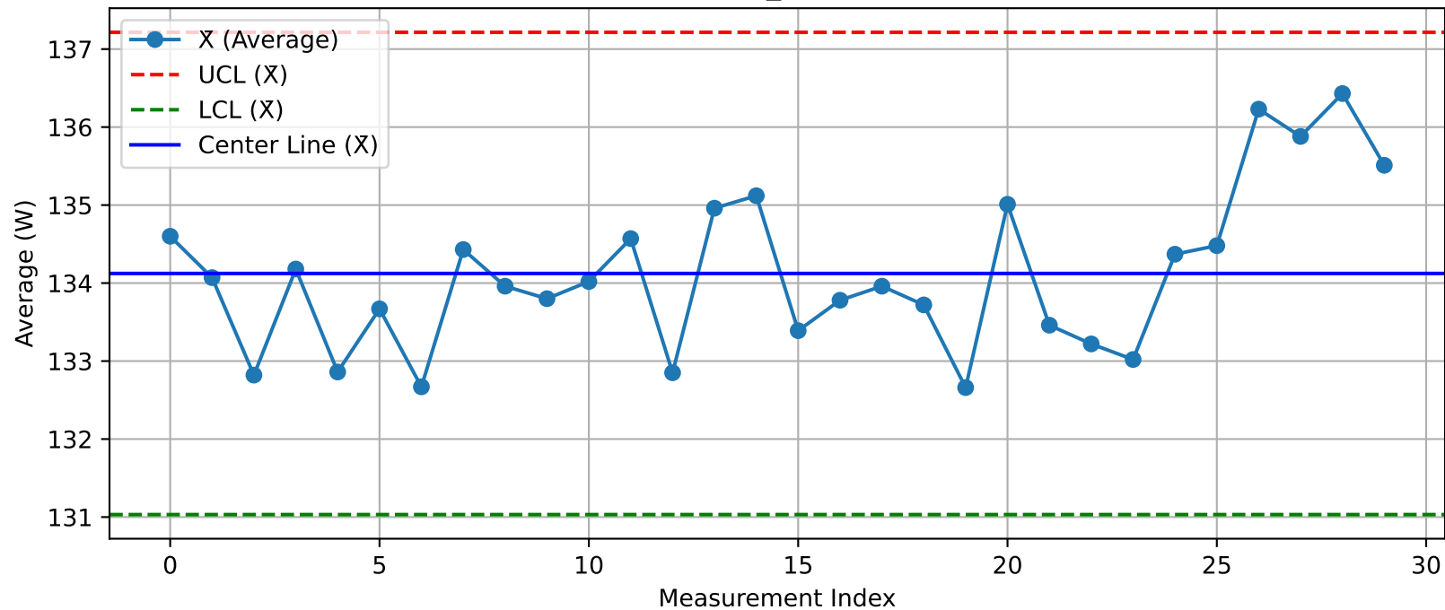
DUT - \bar{X} Chart (T40_Test103@Test.xlsx)
