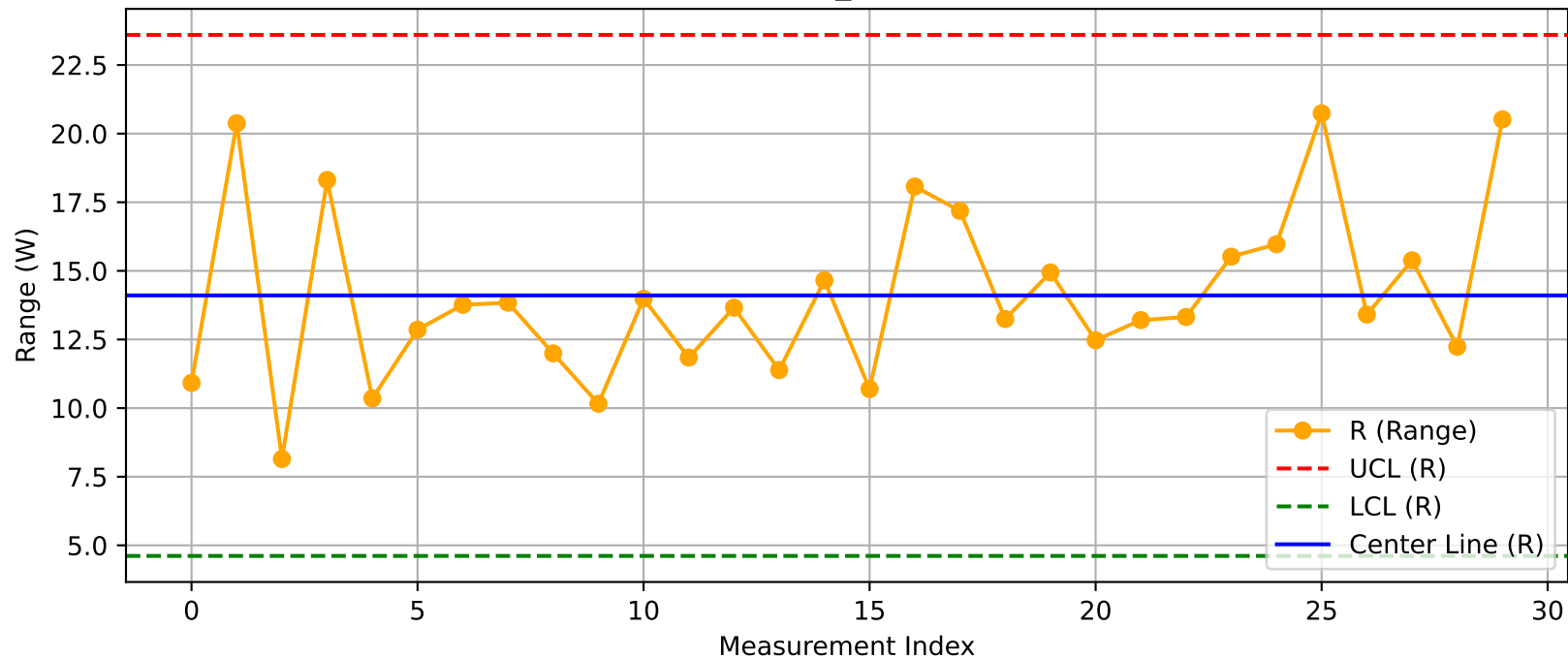
DUT - R Chart (T44_Test100@Test.xlsx)
