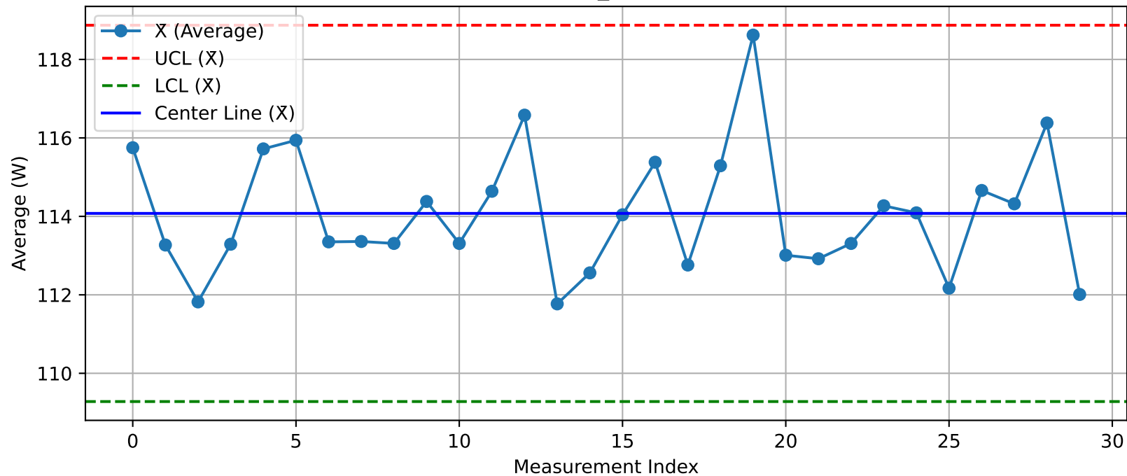
DUT - \bar{X} Chart (T44_Test100@Test.xlsx)
