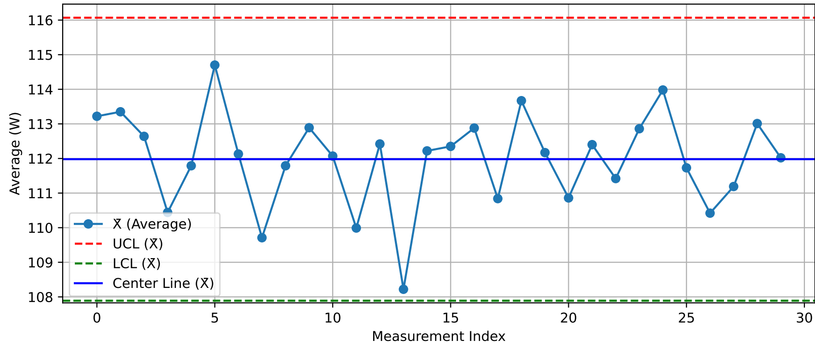
DUT - \bar{X} Chart (T44_Test2O3@Test.xlsx)
