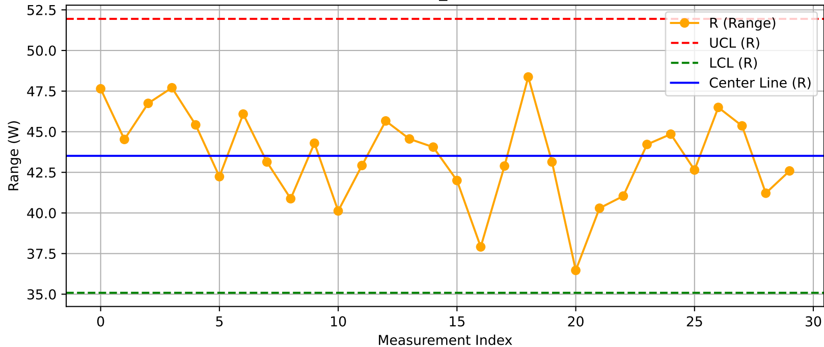
DUT - R Chart (T49_Test200@Test.xlsx)
