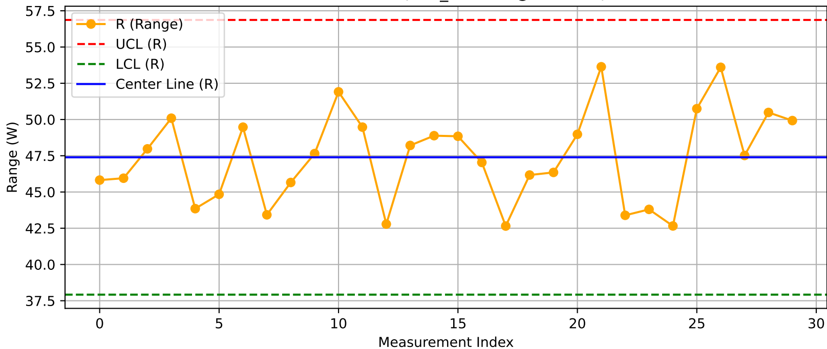
DUT - R Chart (T50_Test2O3@Test.xlsx)
