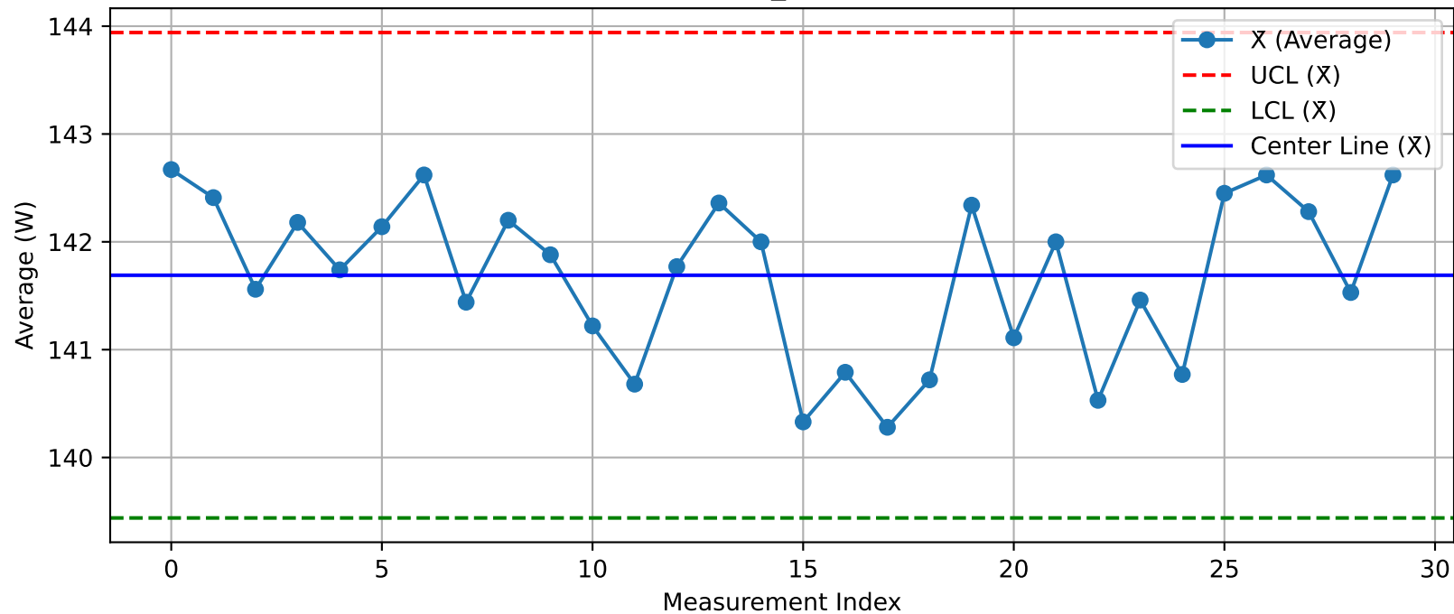
DUT - \bar{X} Chart (T50_Test2O3@Test.xlsx)
