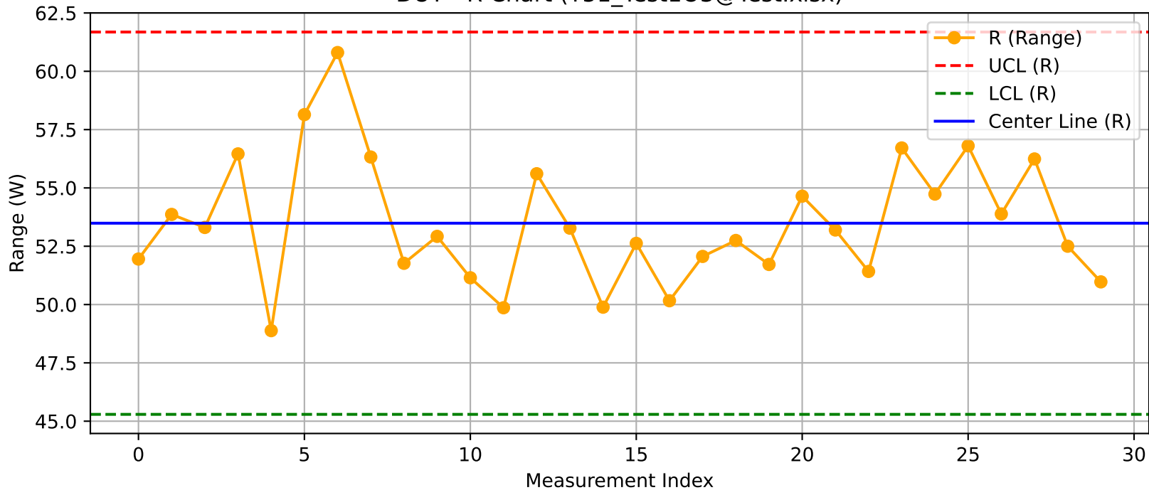
DUT - R Chart (T51_Test103@Test.xlsx)
