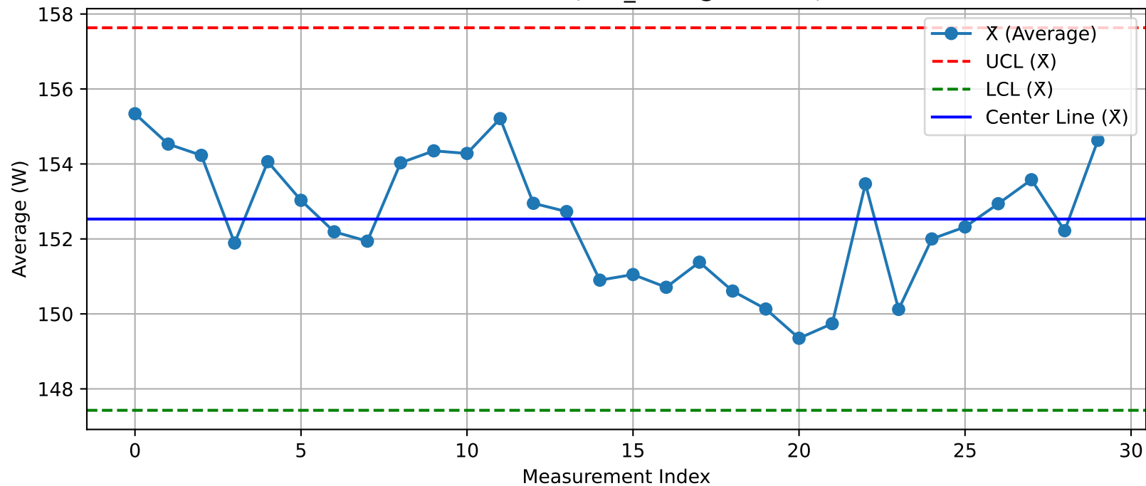
DUT - \bar{X} Chart (T10_Test2@Test.xlsx)
