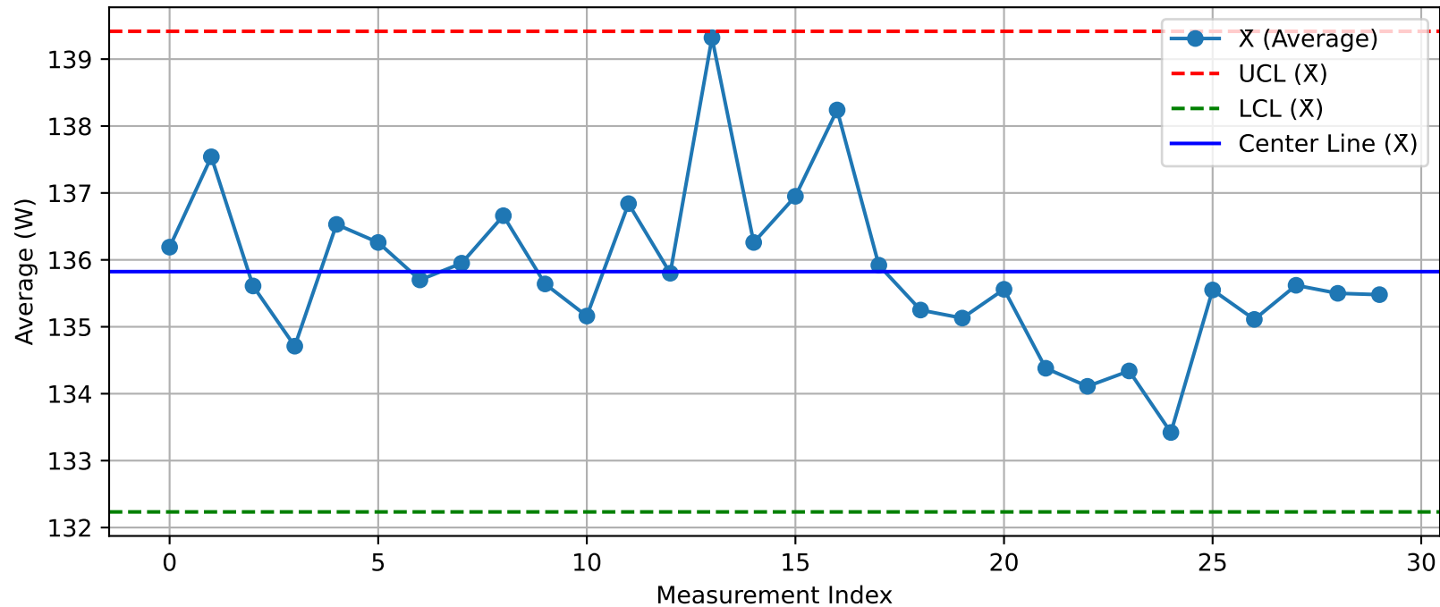
DUT - \bar{X} Chart (T10_Test2_Xint@Test.xlsx)
