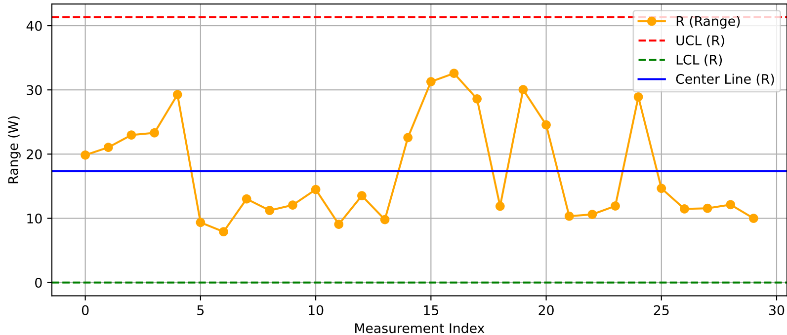
DUT - R Chart (T11_Test1_Xint@Test.xlsx)
