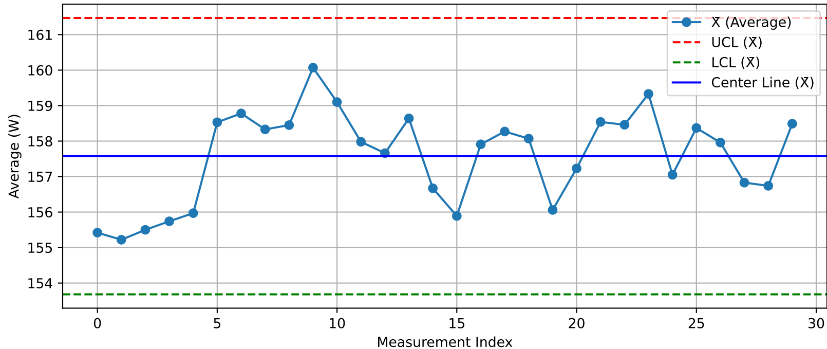
DUT - \bar{X} Chart (T11_Test1_Xint@Test.xlsx)
