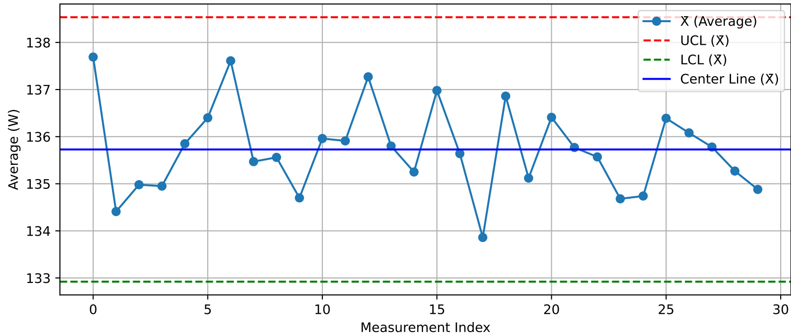
DUT - \bar{X} Chart (T16_Test1@Test.xlsx)
