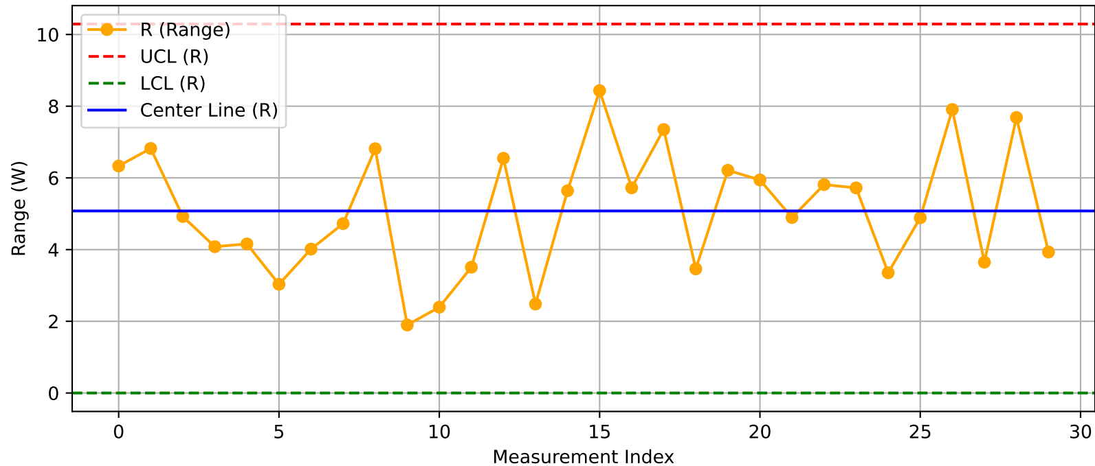
DUT - R Chart (T16_Test2@Test.xlsx)
