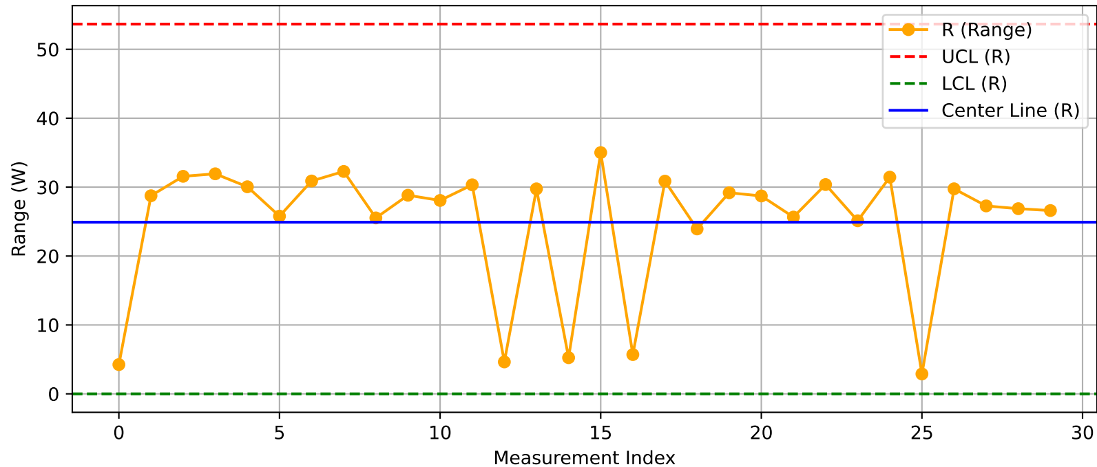
DUT - R Chart (T19_Test1@Test.xlsx)
