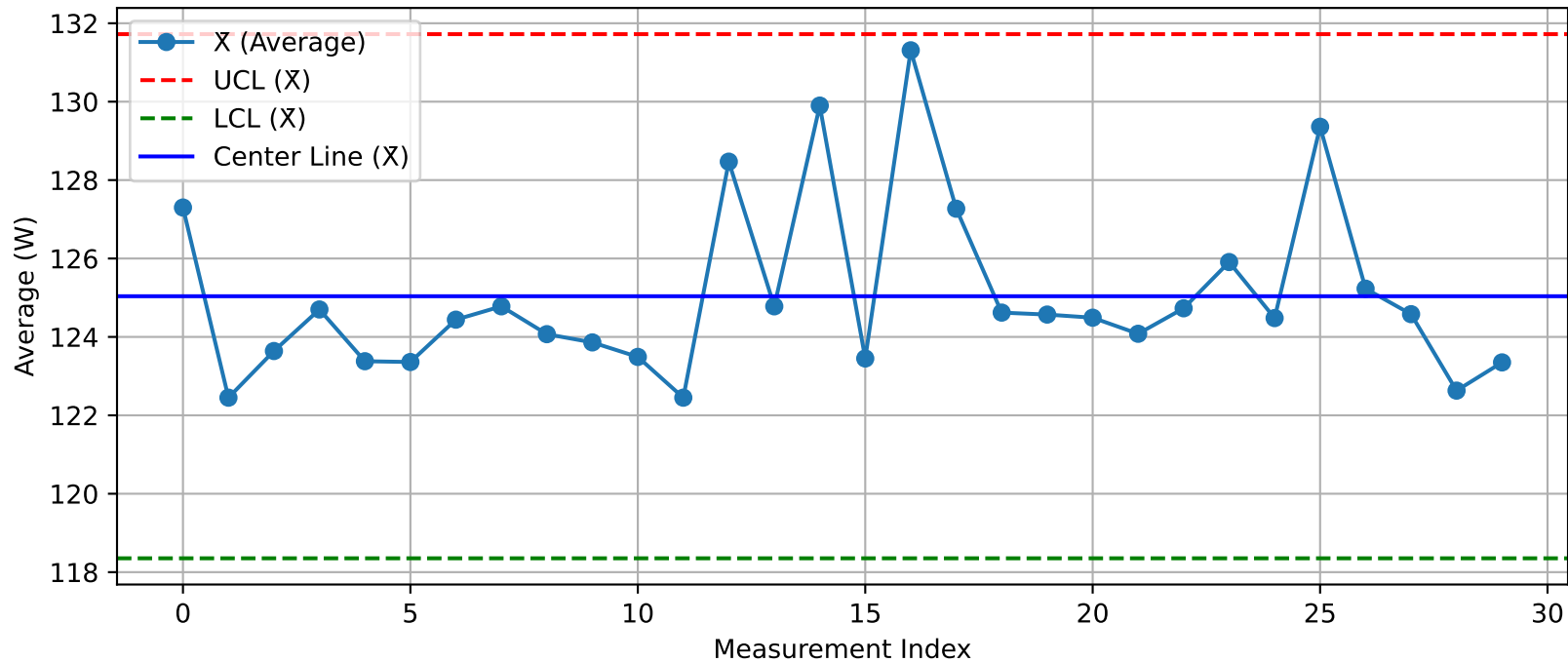
DUT - \bar{X} Chart (T19_Test1@Test.xlsx)
